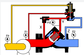
Closed Pilot closed
