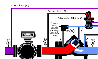
Fully open [no control] Pilot open
