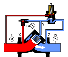
Fully open [no control] Pilot open
