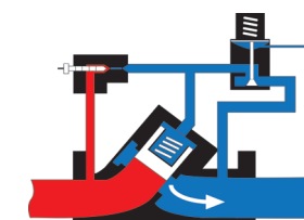
Fully open [no control] Pilot open
