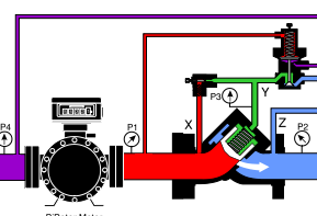
Fully open controlled Pilot partially open
