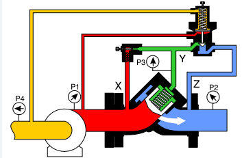
Open [controlled] Pilot partially open
