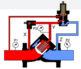
Closed Pilot closed
