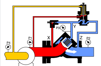
Fully open [no control] Pilot open
