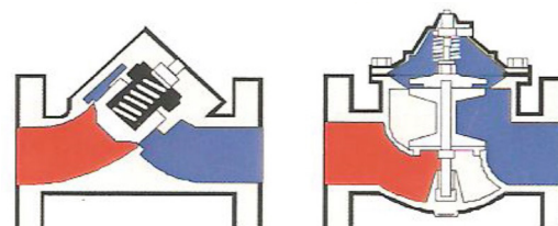
Piston Valve
