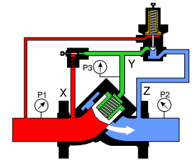
Open [controlled] Pilot partially open
