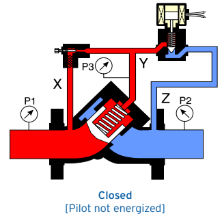
Example BV10 [Normally Closed]:
